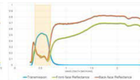
High Performance Double Glazed Unit
